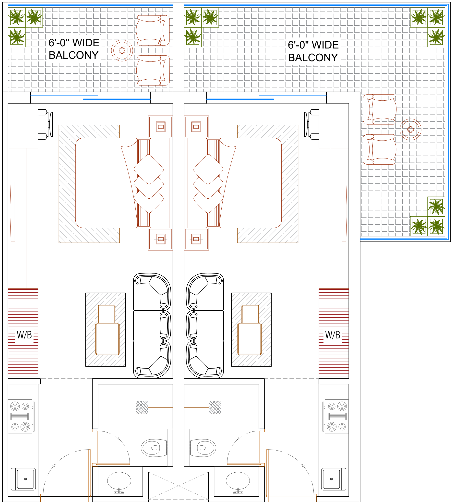
STUDIO - TYPE A
