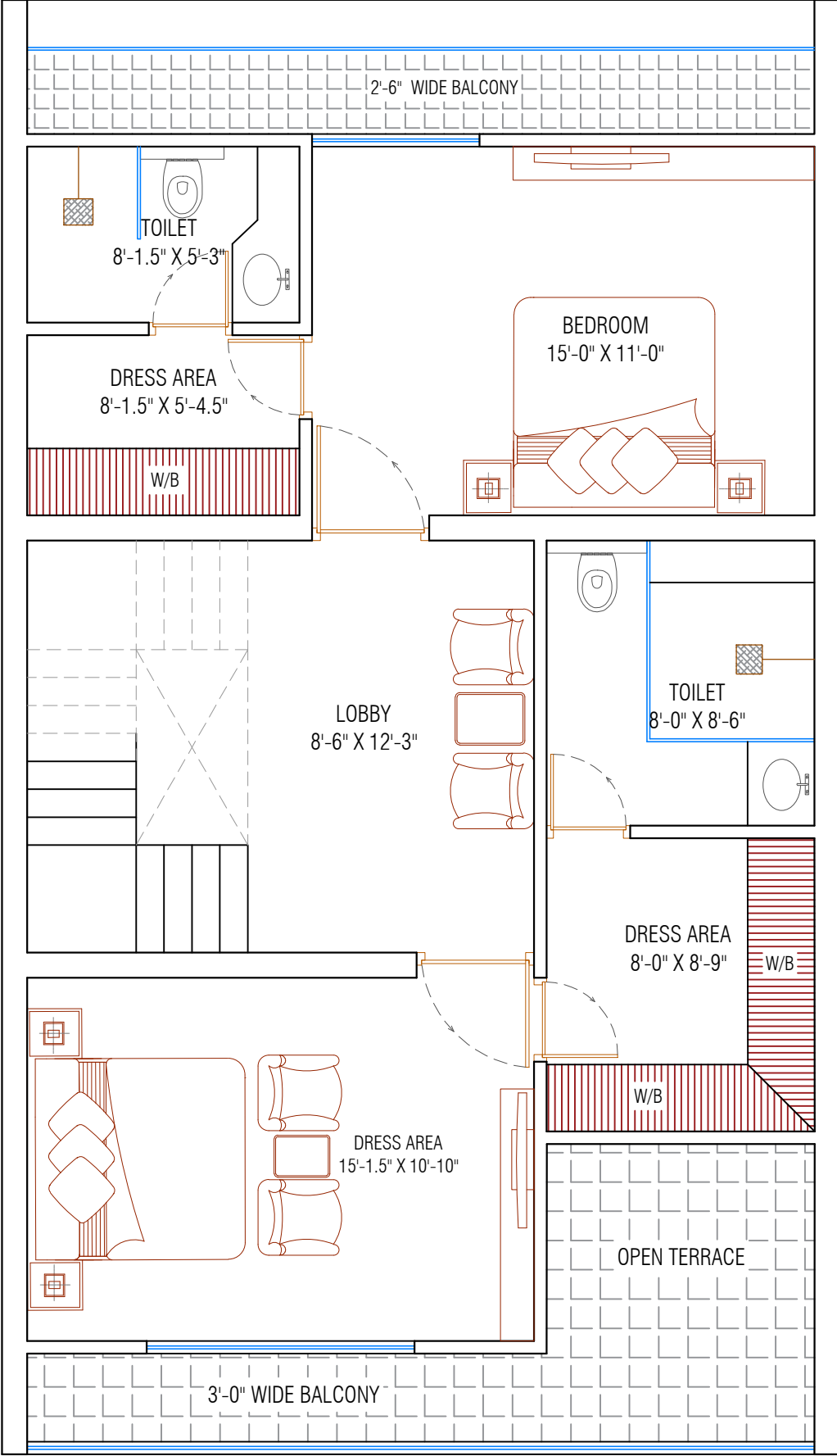
FIRST FLOOR
